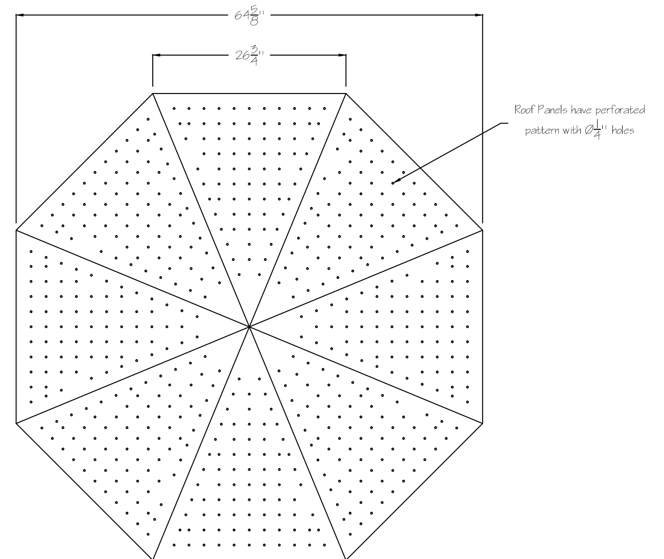
Top View
