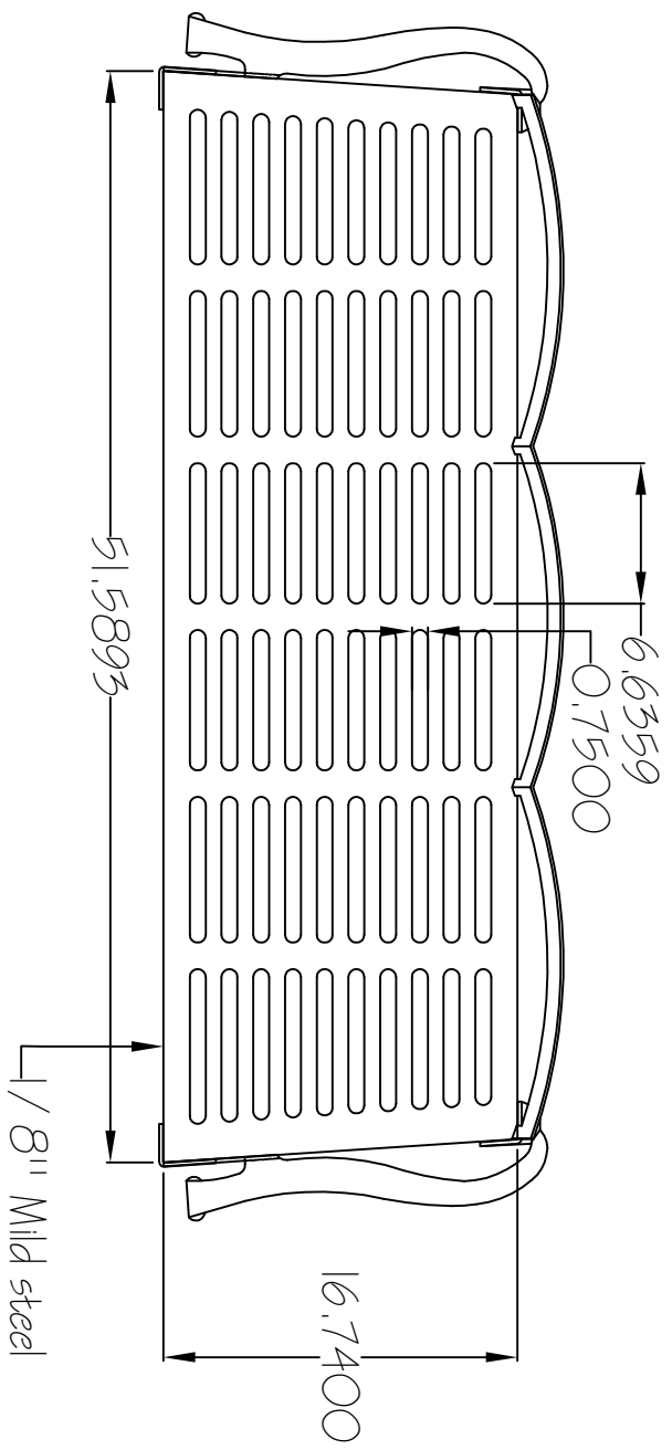
Top View
