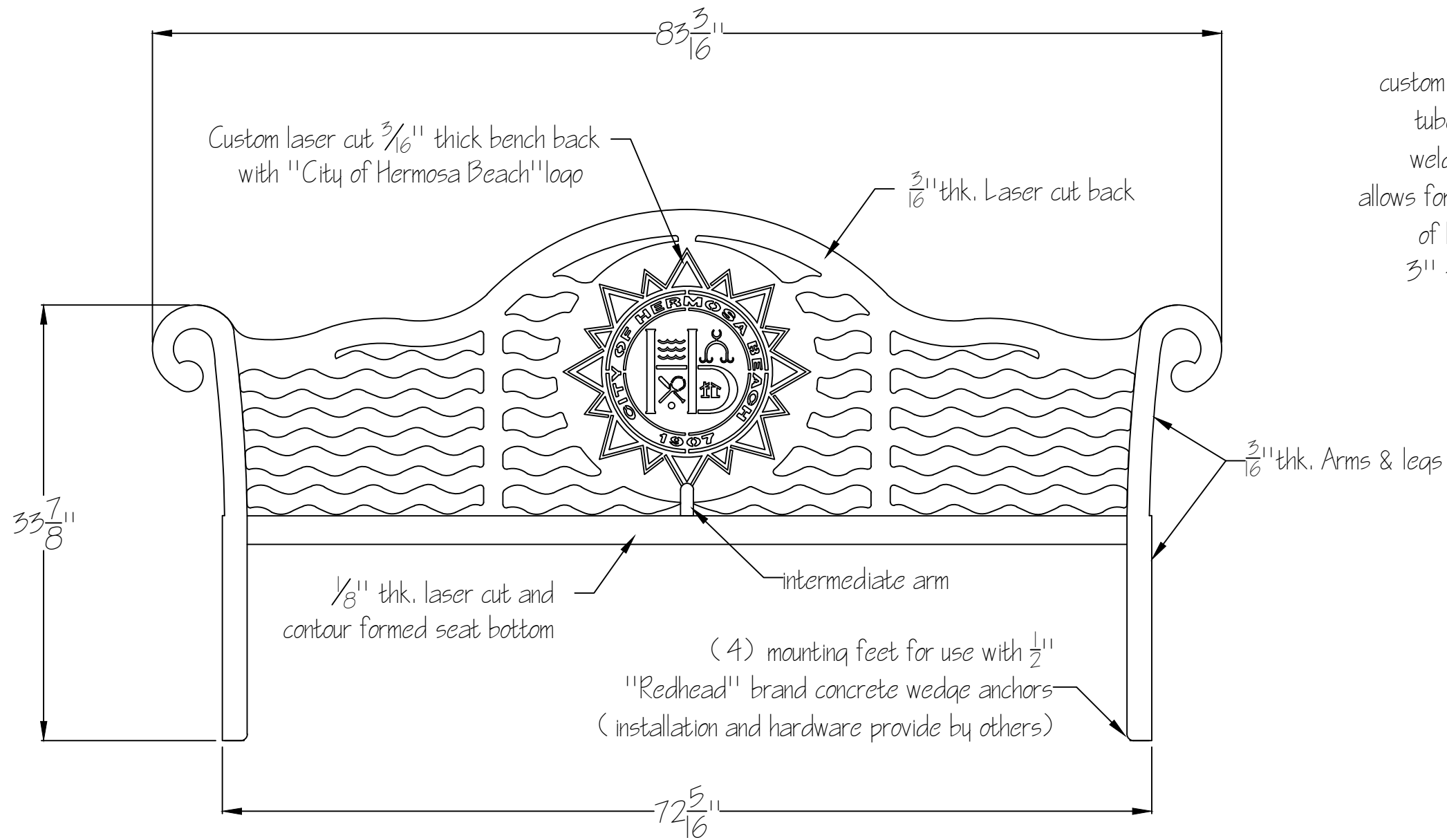
Front Elevation
