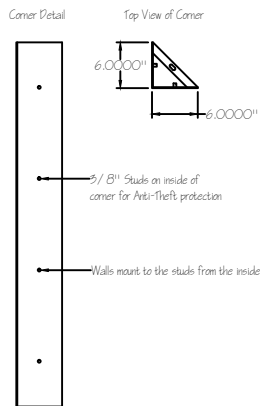
Corner Detail
