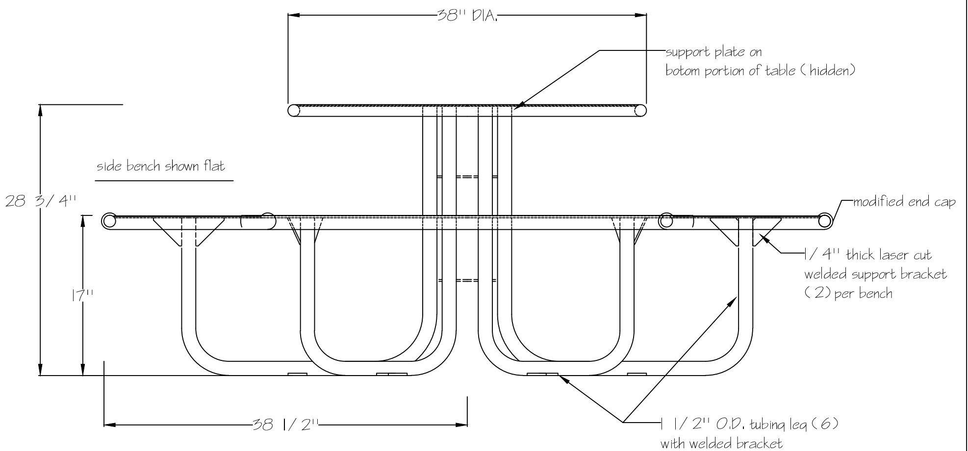
Elevation View
