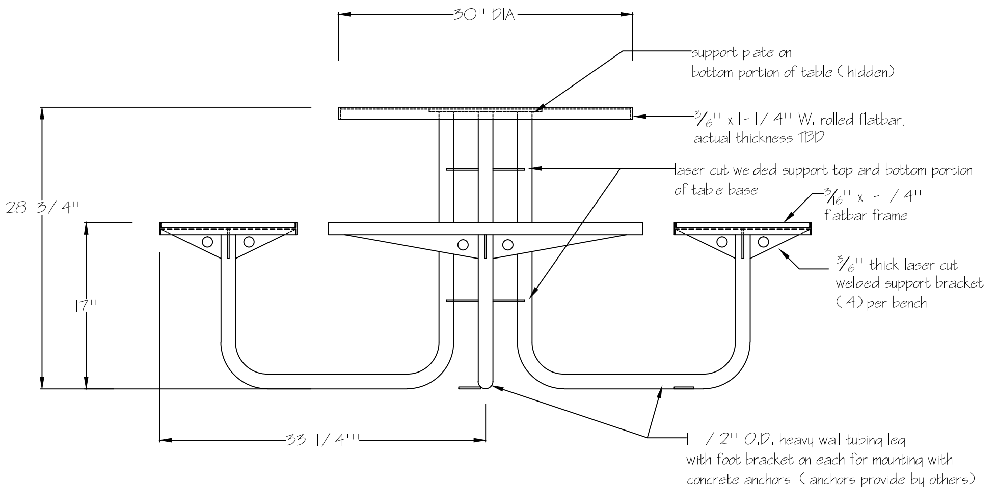
Elevation View
