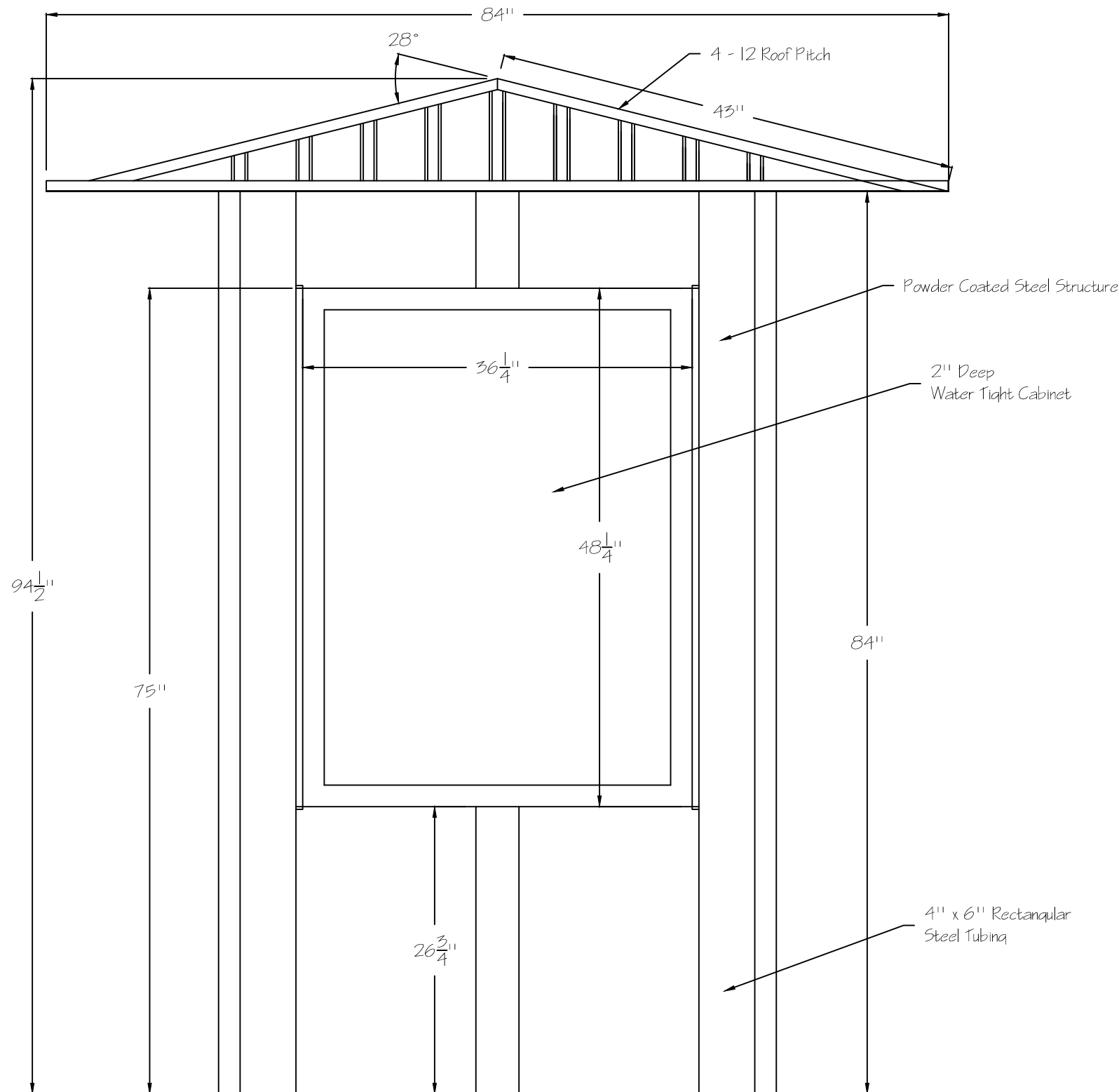
Side View
