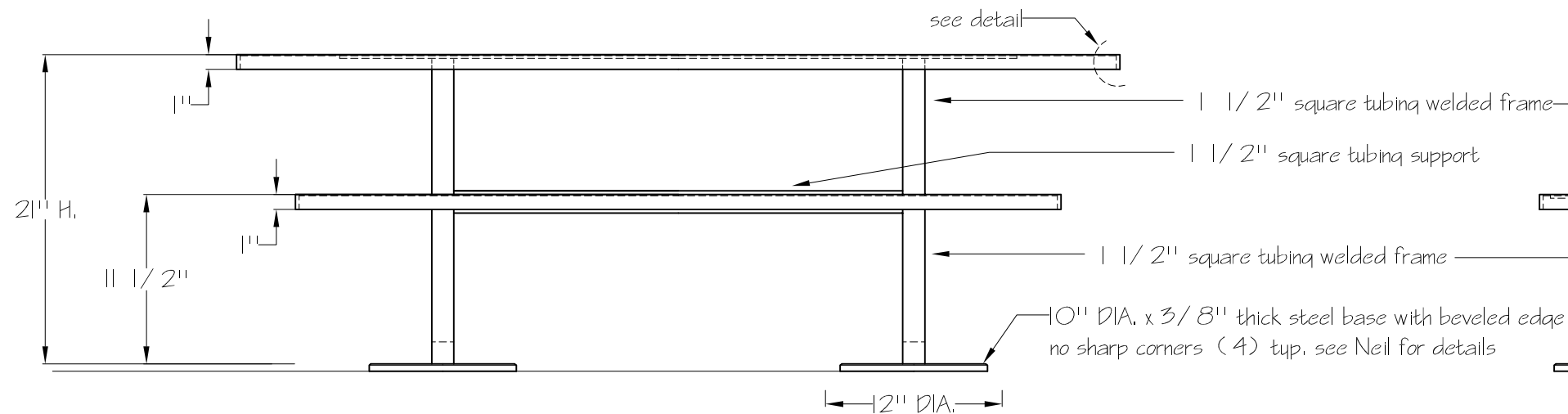
Elevation View
