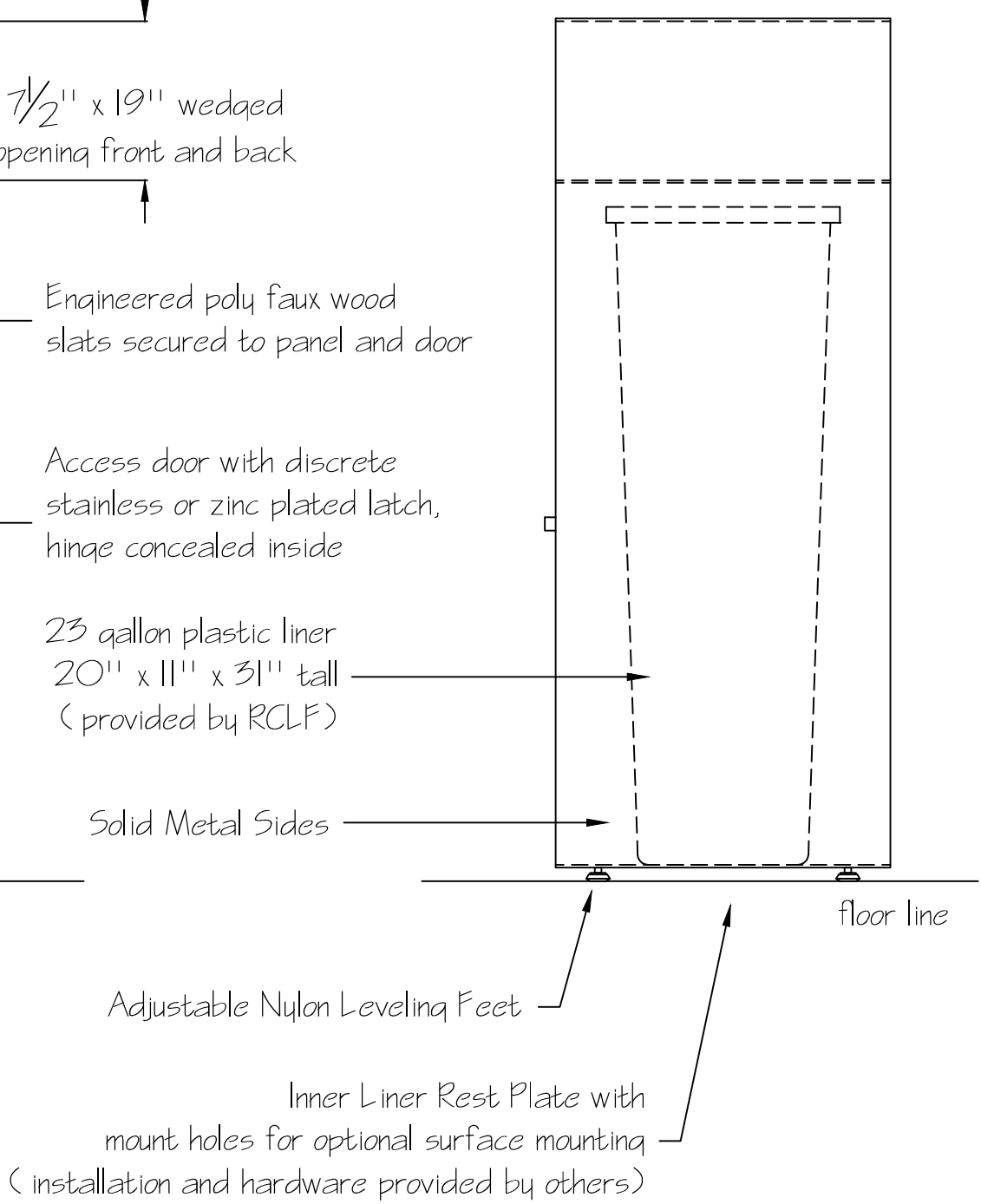
Side View
