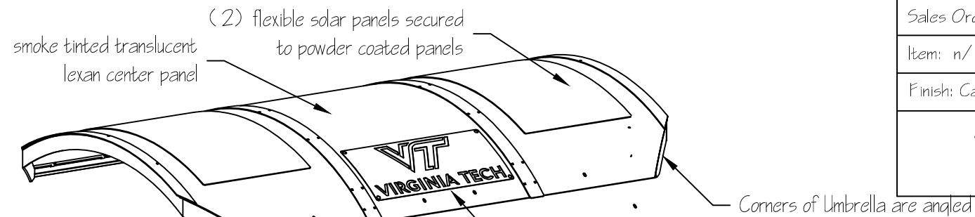
ISO VIEW
