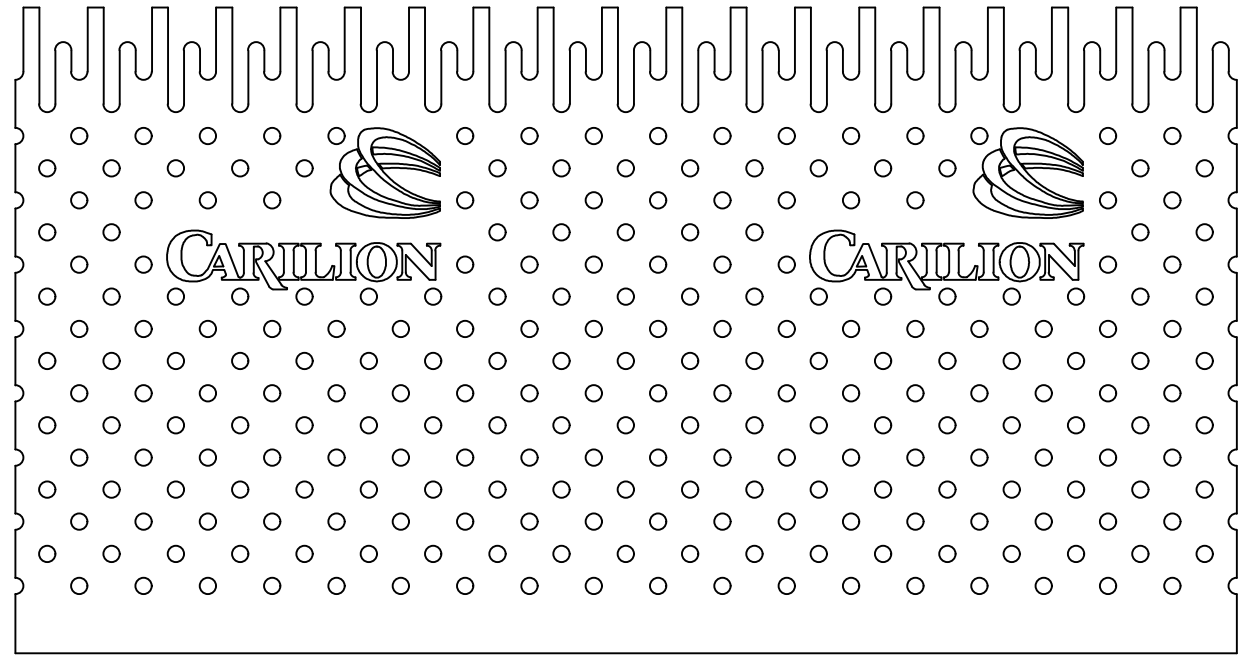
Flat Pattern of Outer Can
